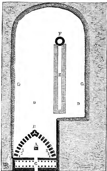
Fig. 386. Ground-plan of a Hippodrome.
